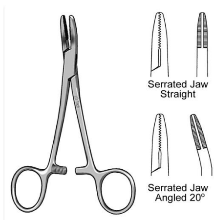
30-561-13 Meniscus Clamp 13.5 cm / 5 3/8" 1X2 teeth
