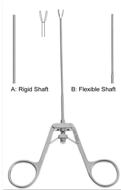
30-559-21 Kleinert-Kutz Tendon Holding Forceps 21 cm / 8 1/4" 1X2 teeth
